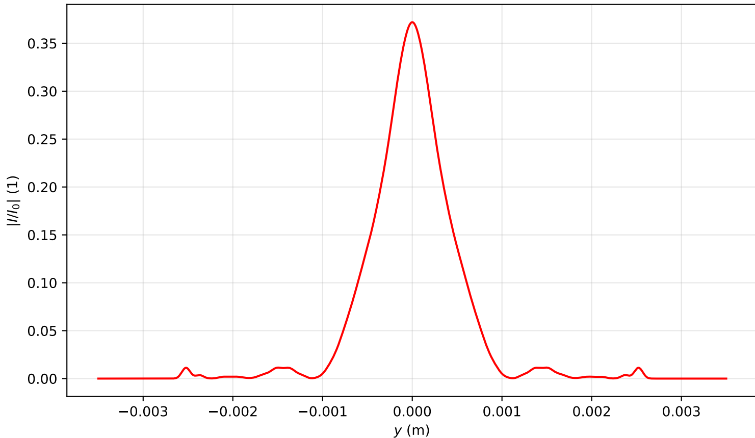
Intensity profile I(x=0, y, z=1.115)/I_0 , P_{in}=3.0P_{cr} , artificial time
